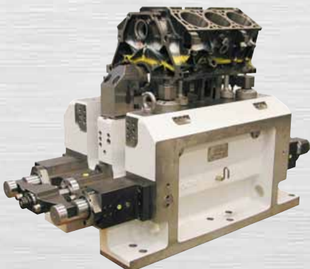
Non-rotating Clamping Devices
